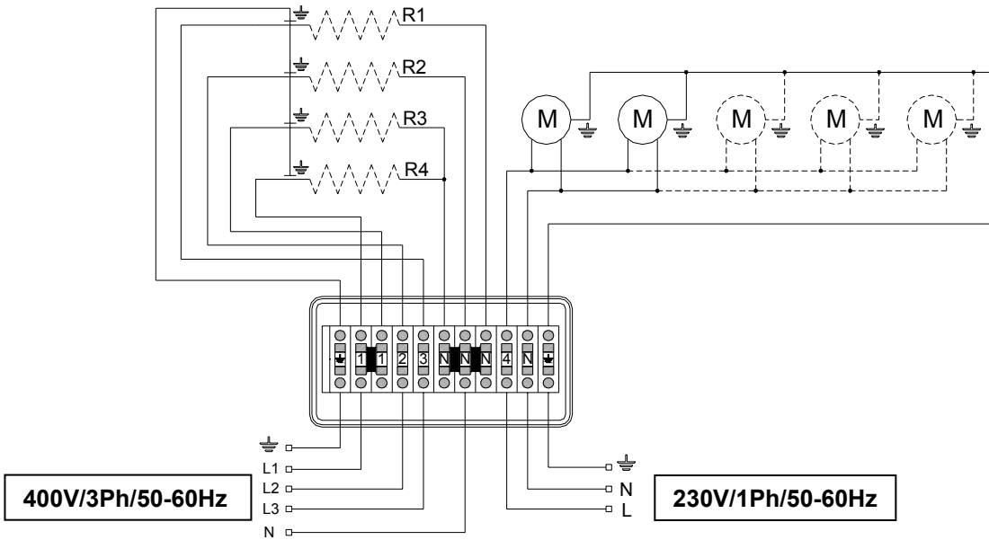
Wiring diagram for heater power at 400V/3Ph/50-60Hz
