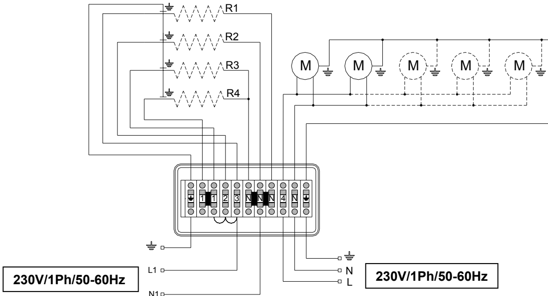
Wiring diagram for heater power at 230V/1Ph/50-60Hz
