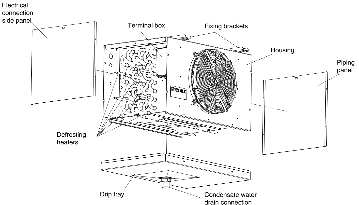
Drawing 6
