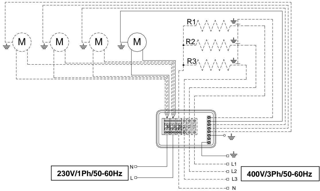
Drawing 5
