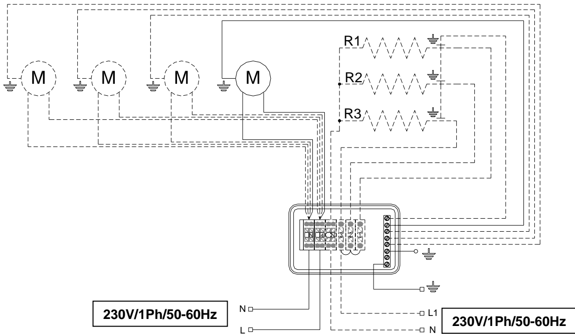
Drawing 5
