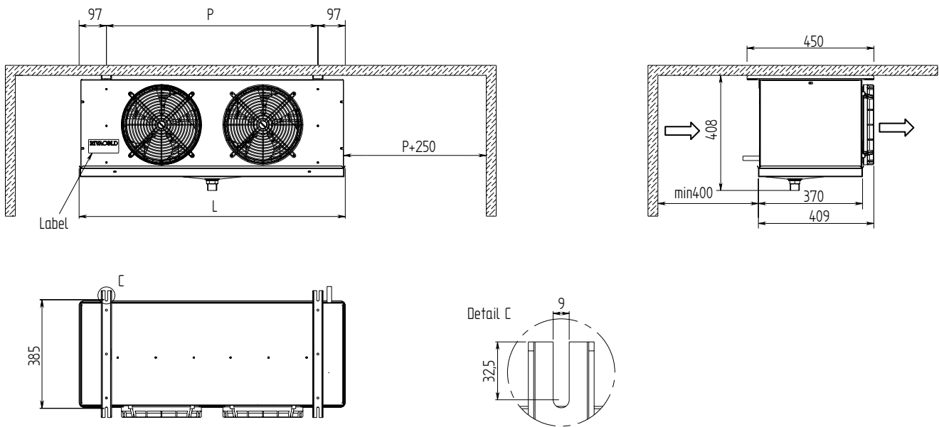
Drawing 1
