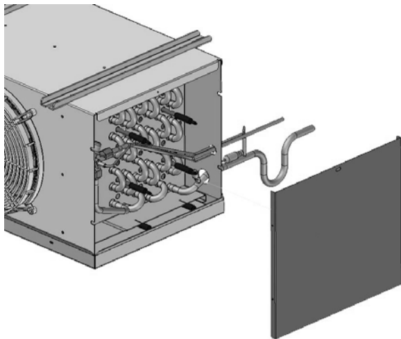
Drawing 2
